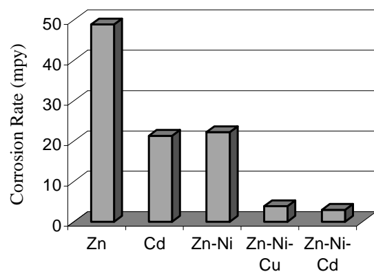
Fig. 1. Comparison Chart of Corrosion rates for different coatings.
