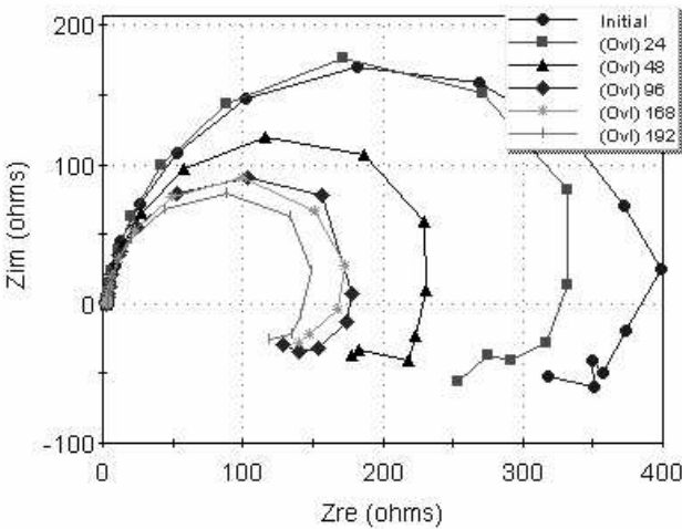
Fig. 1. 304L in 3.55% NaCl in 1.0N HCl at different immersion times (hrs)
