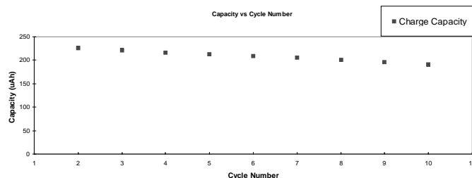
Figure 2: Lithium-ion capacity results for a typical \text{LiCoO}_2 thin film cycled versus a Li metal counter-electrode using liquid electrolyte and a Li metal reference electrode.
