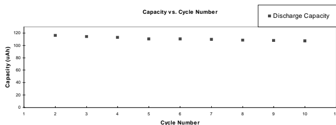
Figure 2: Lithium-ion capacity results for a typical \text{LiCoO}_2 thin film cycled versus a Li metal counter-electrode using liquid electrolyte and a Li metal reference electrode.
