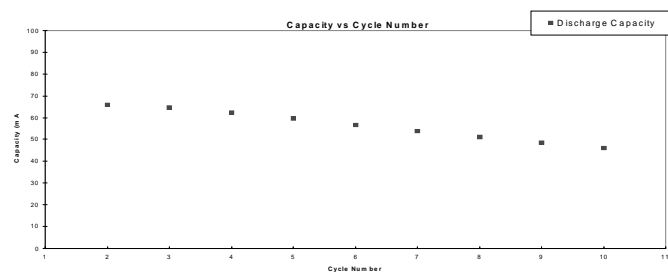
Figure 4: Lithium-ion capacity results for a typical thin film battery of the type, \text{LiCoO}_2 | PAN, EC, PC, \text{LiN}(\text{CF}_3\text{SO}_2)_2 | \text{SnO}_2 .
