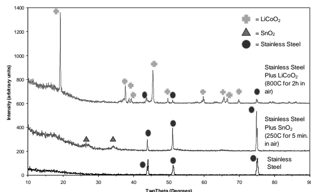
Figure 1 : XRD of the substrate and thin films prior to electrochemical cycling.
