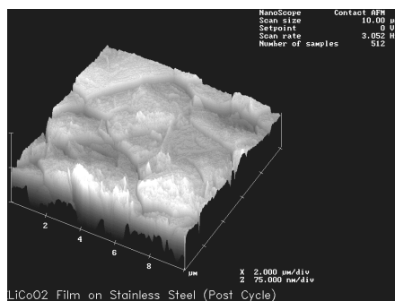
Figure 5: AFM image showing the surface of the \text{LiCoO}_2 thin film after 10 cycles (liquid electrolyte, Li metal counter-electrode).
