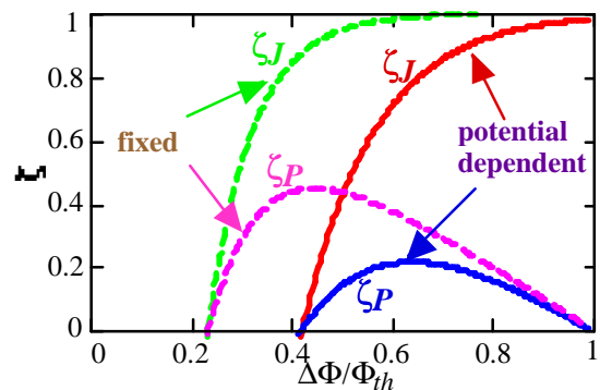
Figure 2. Comparison of current and power efficiency curves using potential dependent or fixed boundary conditions. \zeta is efficiency.
