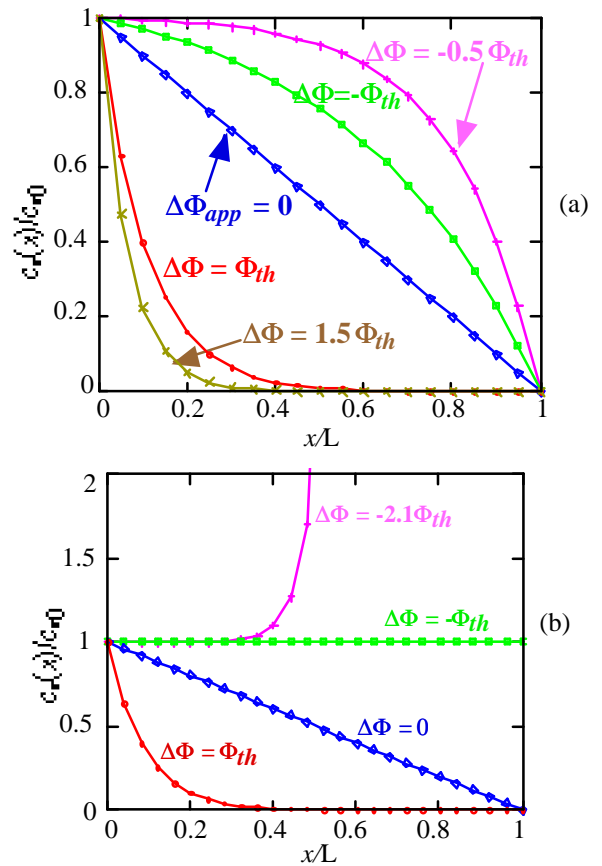
Figure 1. Electron concentration profile with (a) fixed boundary conditions and (b) potential dependent boundary conditions. \Delta\Phi is the voltage drop across the MIEC and \Phi_{th} is the theoretical (Nernst) potential.
